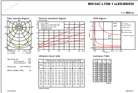
IFGU1_BN126CL15001xLED48S830
