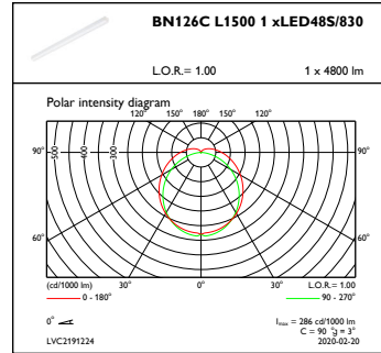
OFPC1_BN126CL15001xLED48S830
