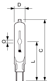
CDM-TC Elite 50W/930 G8.5
