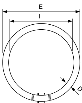
TL5-C 40W/840
